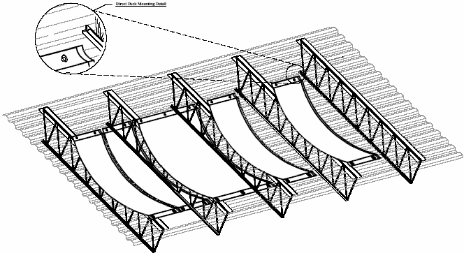
Direct Deck Mounting Detail
