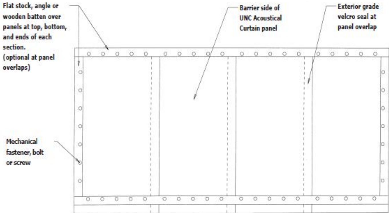
OUTDOOR INSTALLATION OF ACOUSTICAL CURTAIN PANELS ON WALL OR STRUCTURAL STEEL FRAMEWORK
