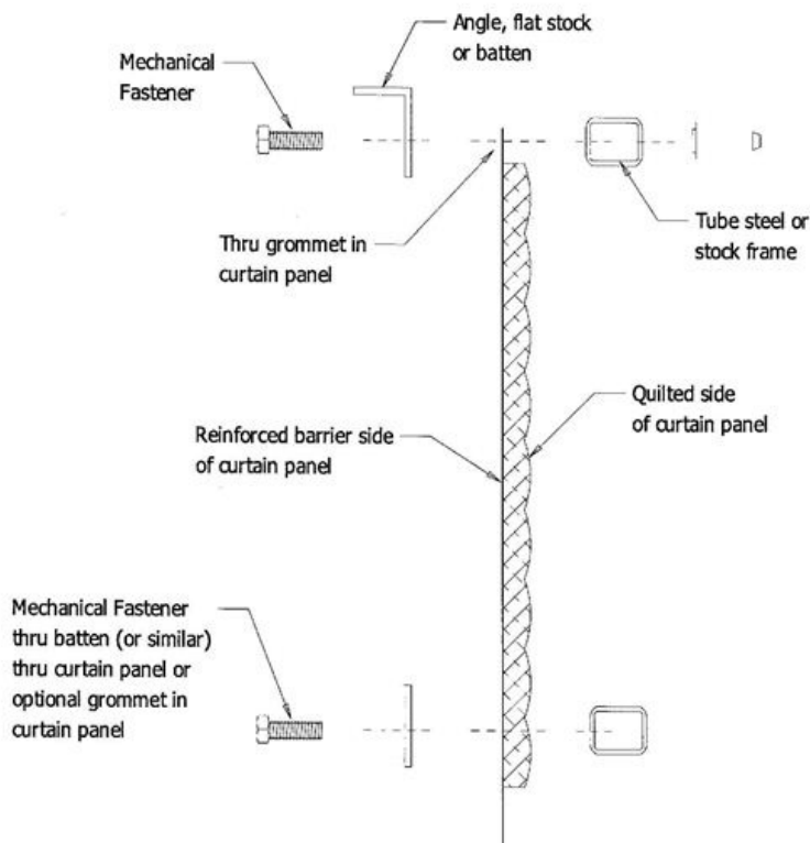
OUTDOOR INSTALLATION OF ACOUSTICAL CURTAIN PANELS ON WALL OR STRUCTURAL STEEL FRAMEWORK
