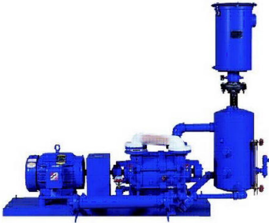
Typical Vacuum Pump
